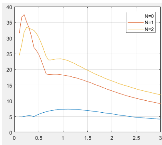
Fig 1. Maximum external displacements for impulse loads at different \omega
