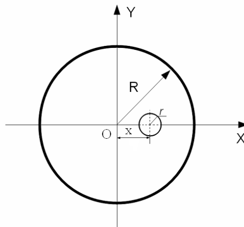
Fig.1. Calculation scheme for determining natural frequencies and oscillations forms of plates with a hole
