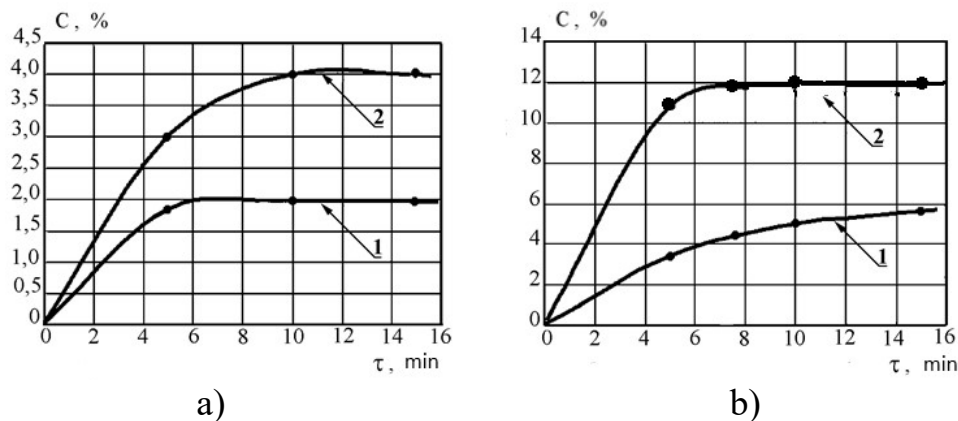
Figure 2 – The amount of dry matter output C , % depending on the duration \tau , min of processing in pulsation devices:
