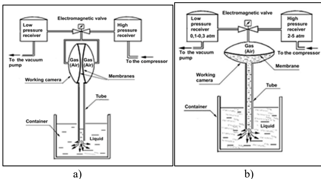
Figure 1 – Schematic diagram of the impact type pulsating disperser (a) and the cavitation type pulsating disperser (b)
